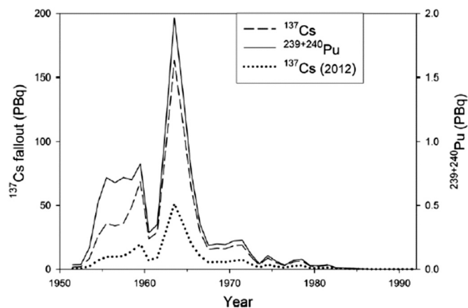
Fig. 1. ^{137}\text{Cs} and ^{239+240}\text{Pu} radiogenic fallout from nuclear weapons testing (from Hancock et al., 2014).
