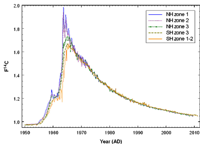
Fig. 2. Atmospheric ^{14}\text{C} concentration changes across the Earth (NH1 is Northern Hemisphere zone 1, being most northerly, and SH1-2 Southern Hemisphere Zone 1–2 most southerly) (from Hua et al., 2013).
