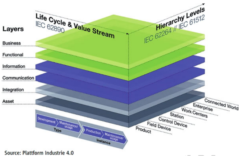
Source: Plattform Industrie 4.0 Fig. 3 Reference architectural model industrie 4.0 (RAMI 4.0)
